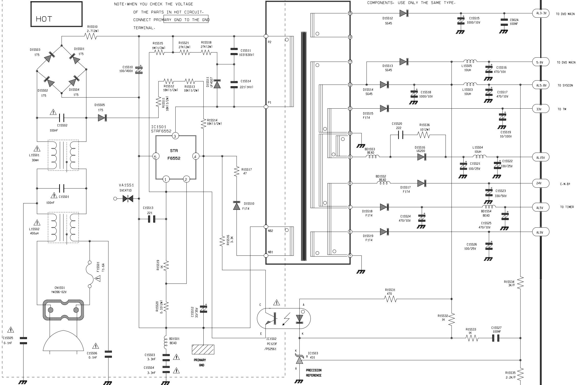
SMPS BLOCK
