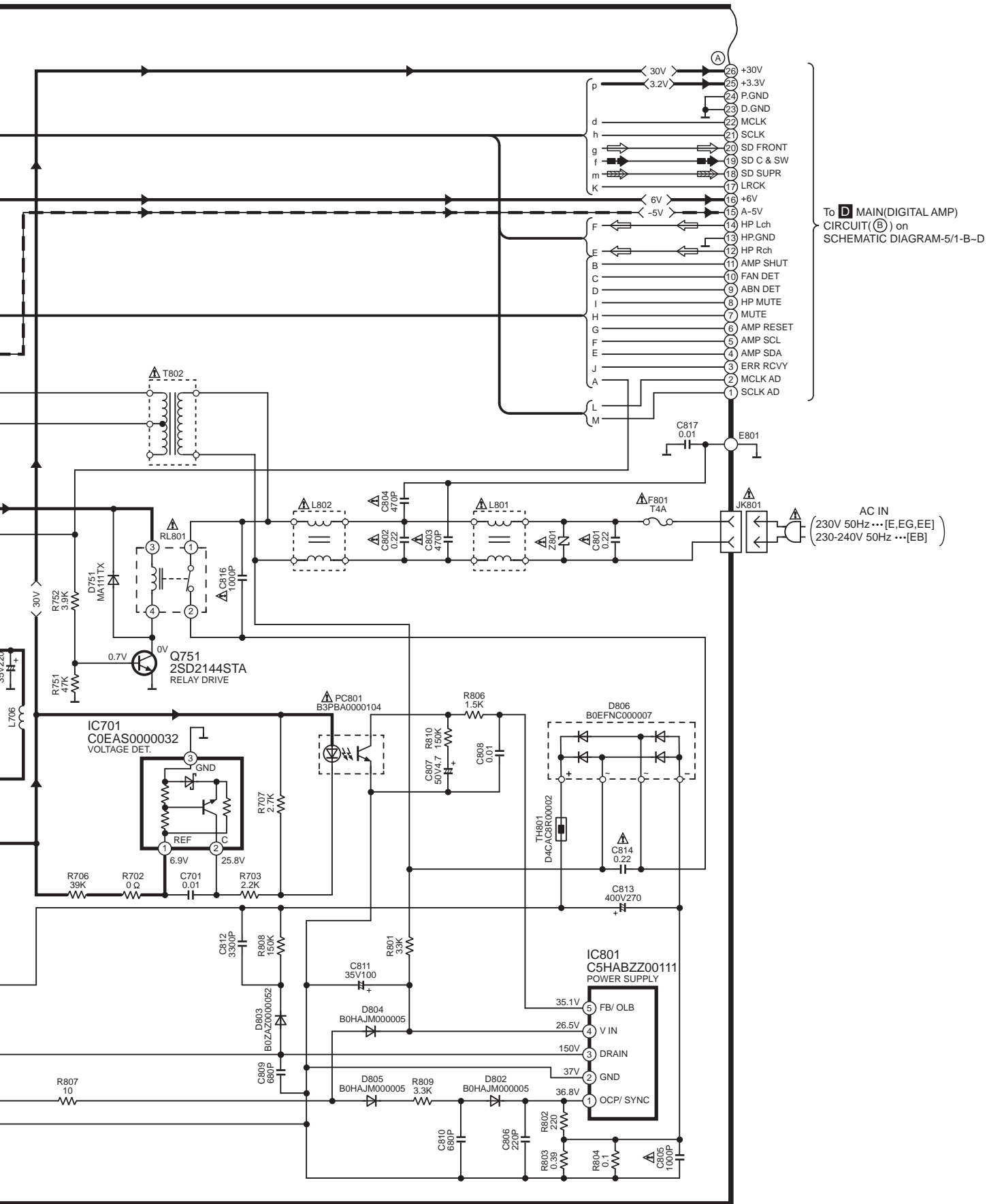
SA-DT310(E,EB,EG,EE) MAIN(SYSTEM) CIRCUIT DIAGRAM
