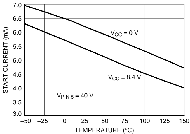
Figure 21. Start Current versus Temperature
