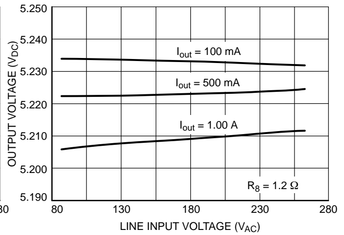
Figure 30. Charger Line Regulation
