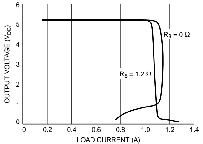
Figure 32. Charger Load Regulation
