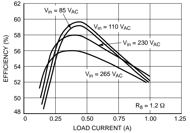
Figure 36. Charger Efficiency
